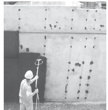
Fig. 3: Spray-applied dampproofing to foundation wall.
