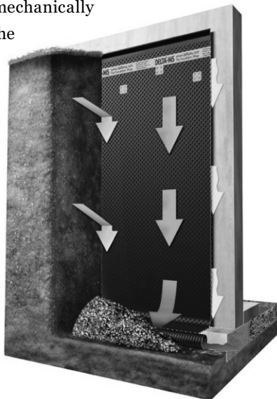
Fig. 5: Dimple membrane system.
