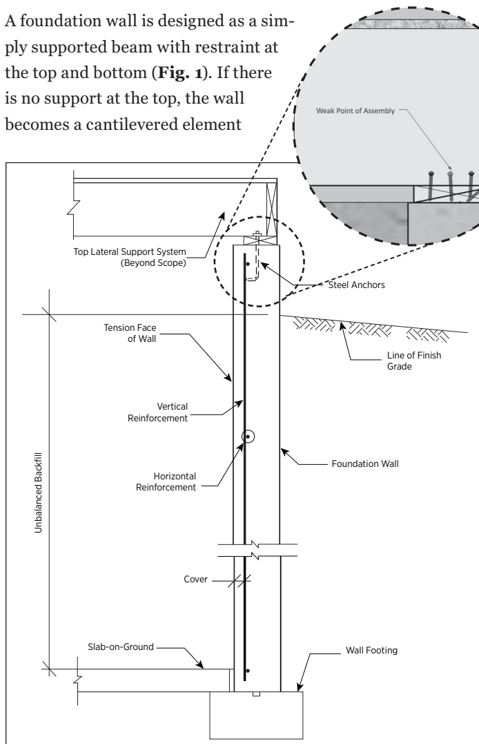
Fig. 1: Typical simply supported foundation wall.
