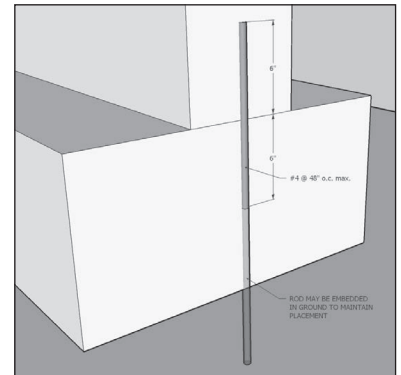
Fig. 4: Typical rebar dowel footing connection.
