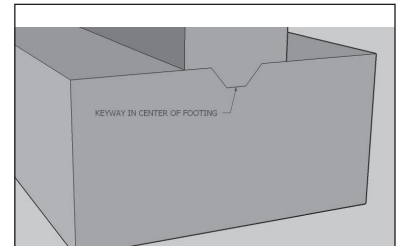
Fig. 3: Typical keyway footing connection.
