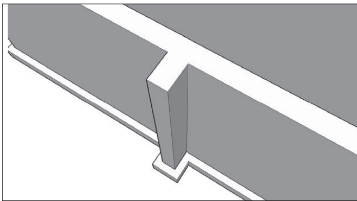
Fig. 6: A counterfort monolithic with the foundation wall will support longer wall lengths like an offset or corner.
