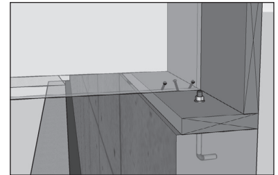
Fig. 2: Typical completed deck connection.
