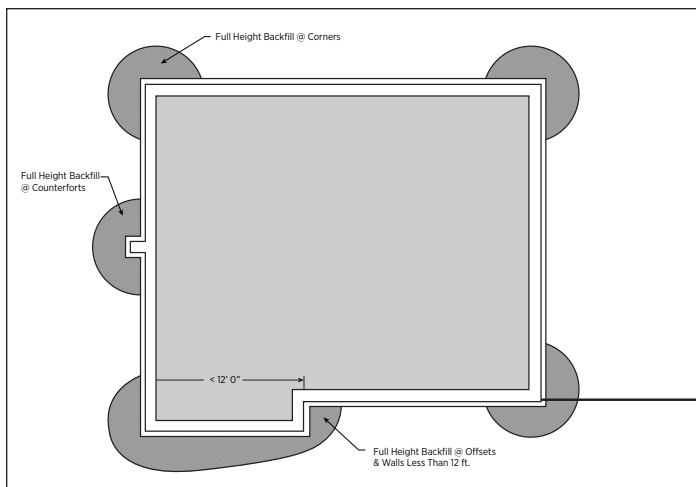
Fig. 5: Common allowable areas for full-height backfill.
